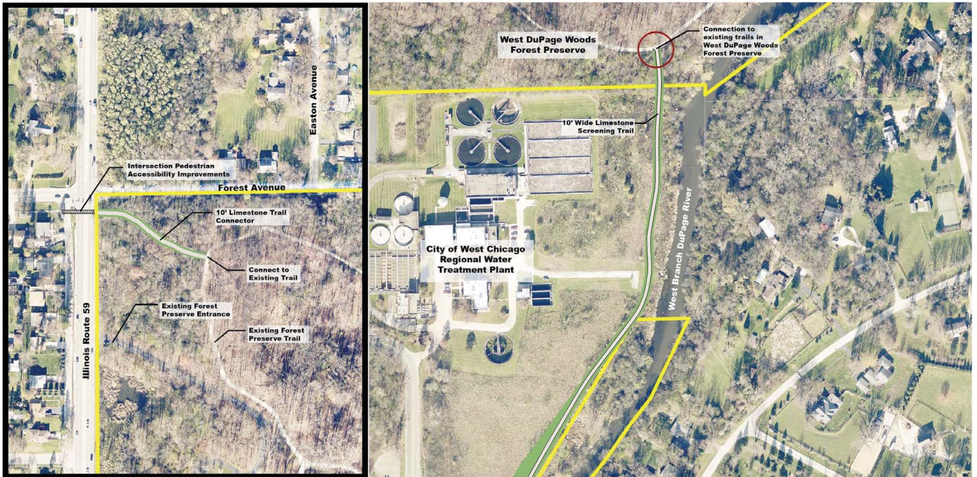
IL Route 59 and Forest Ave Intersection Detail
